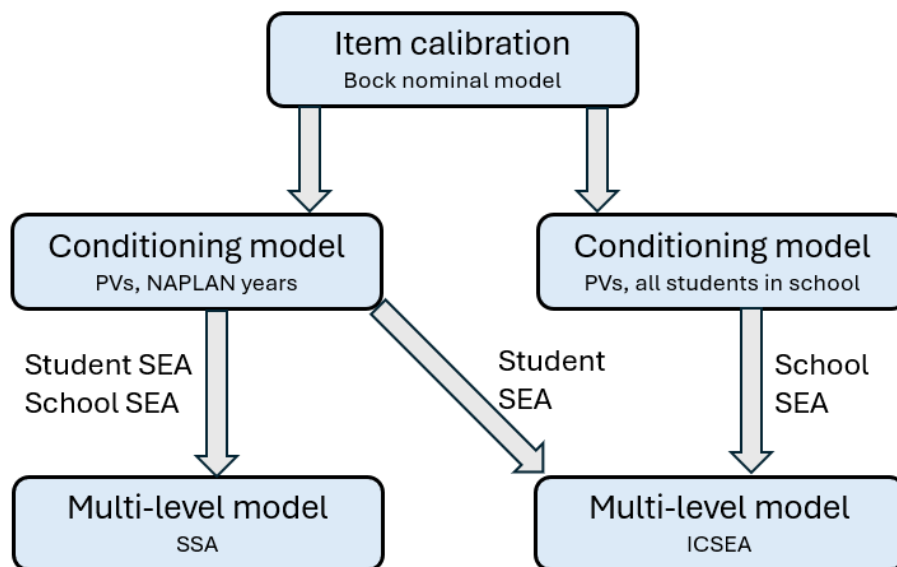
Figure 1: SSA and ICSEA process overview
