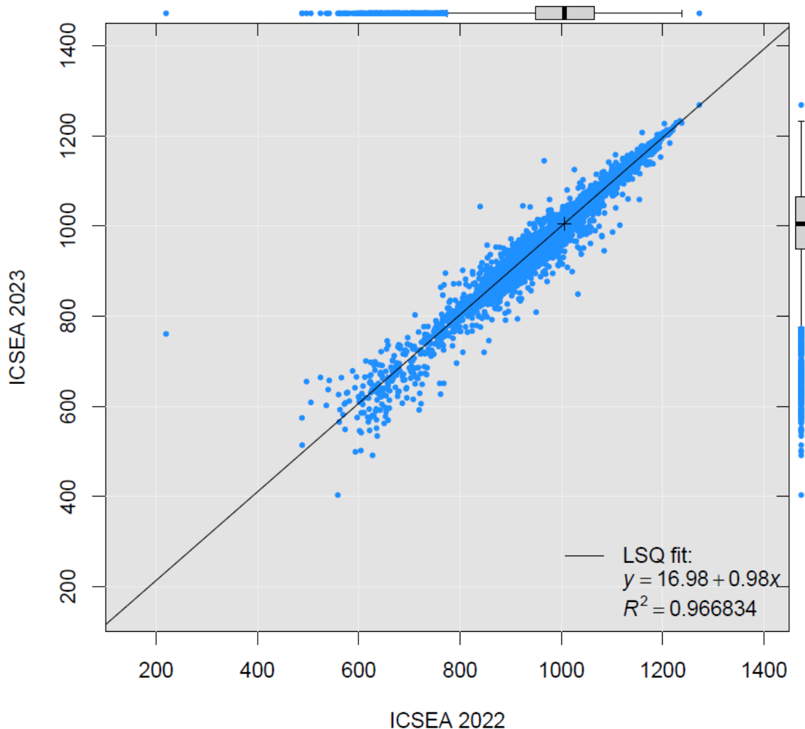
Figure 7: ICSEA 2022 compared with ICSEA 2023
