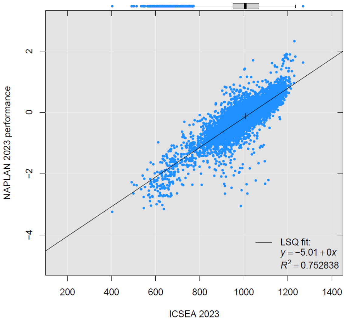
Figure 8: ICSEA 2023 compared with NAPLAN performance
