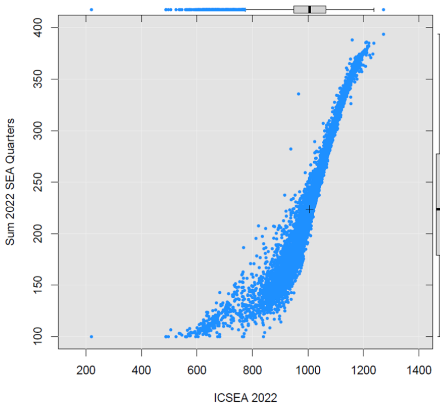
Figure 9: ICSEA 2022 compared with sum of SEA quarters
